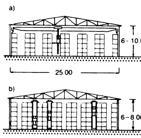
⑩ a) Universal store with overhead gantry crane b) Warehouse with built-in pallet racks
